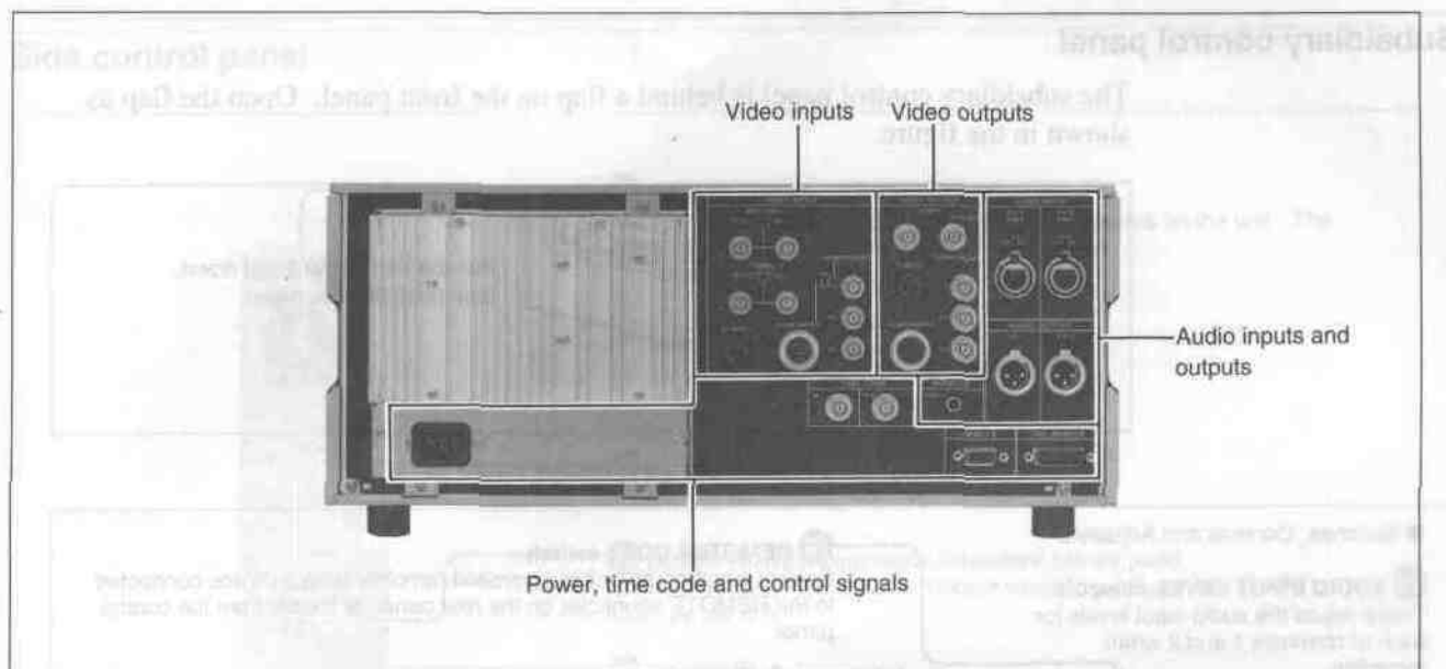
Rear Panel
