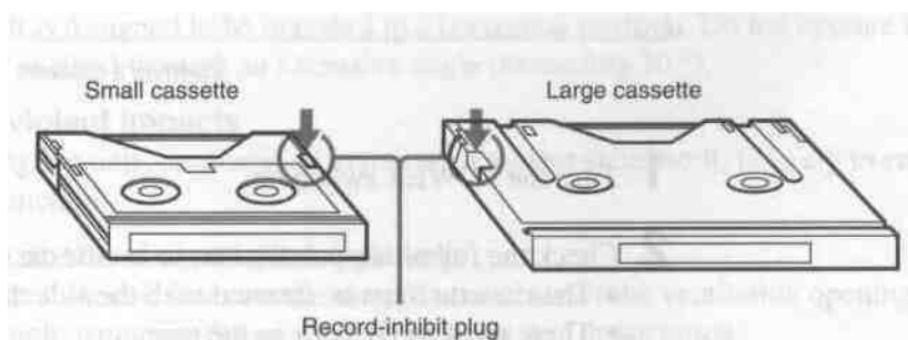
Record-inhibit plug
