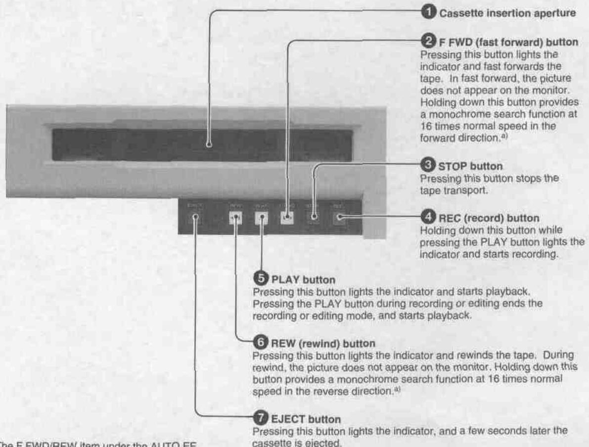
Tape transport section
