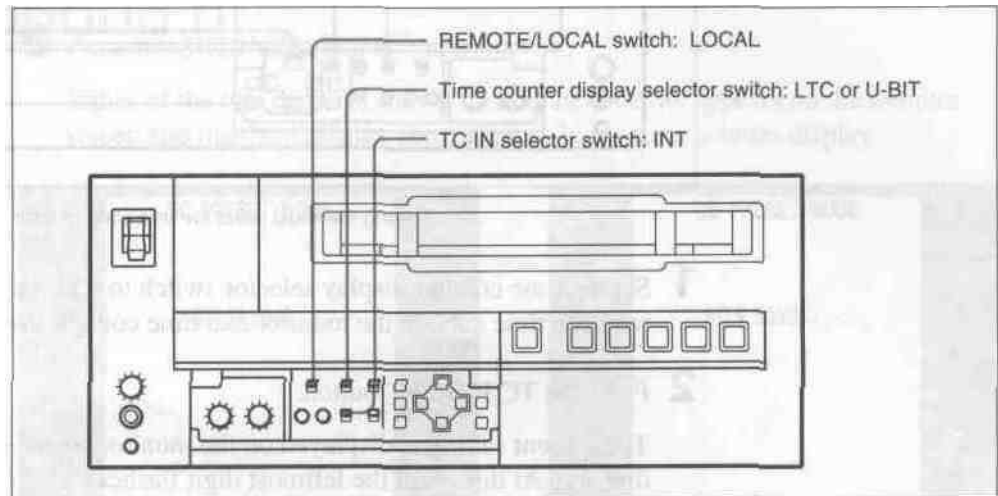
Switch settings
