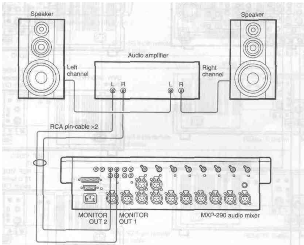
Connecting speakers
